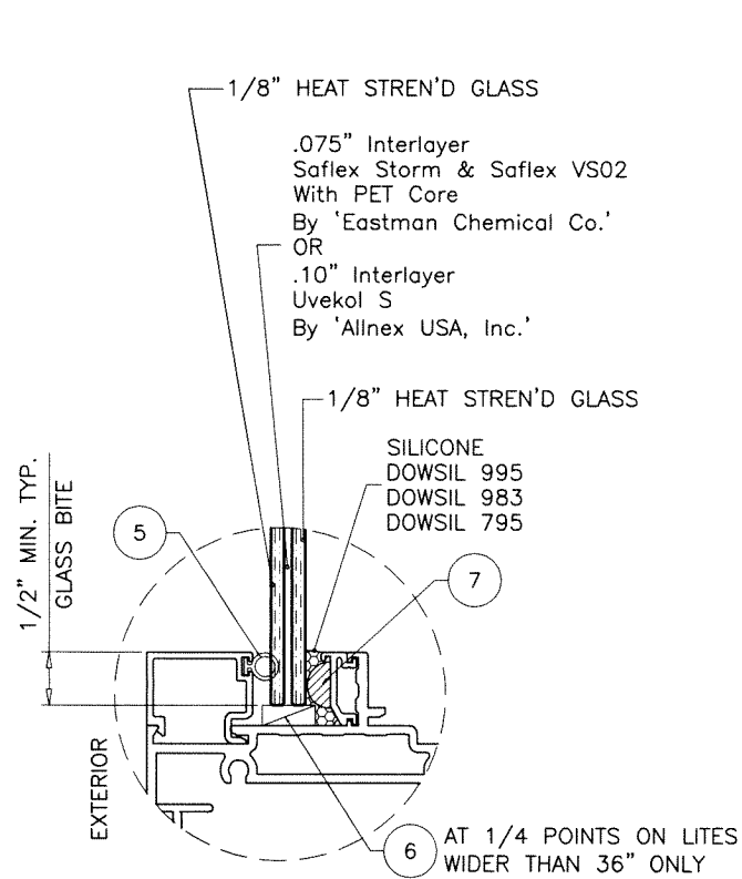
GLASS TYPE 'A' 5/16" OVERALL LAM. GLASS
