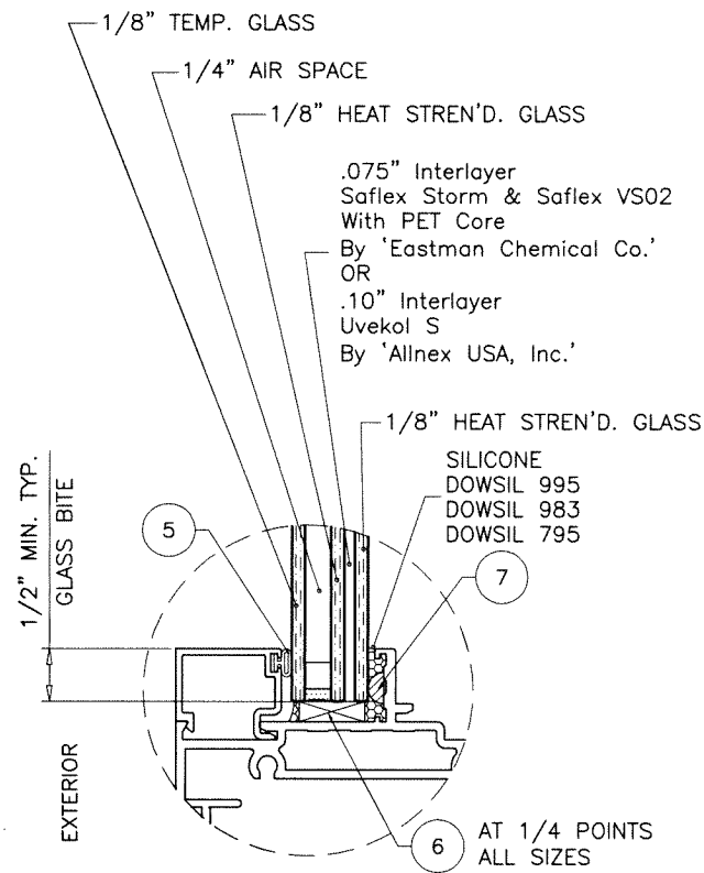
GLASS TYPE 'Ai' 11/16" OVERALL LAM. GLASS
