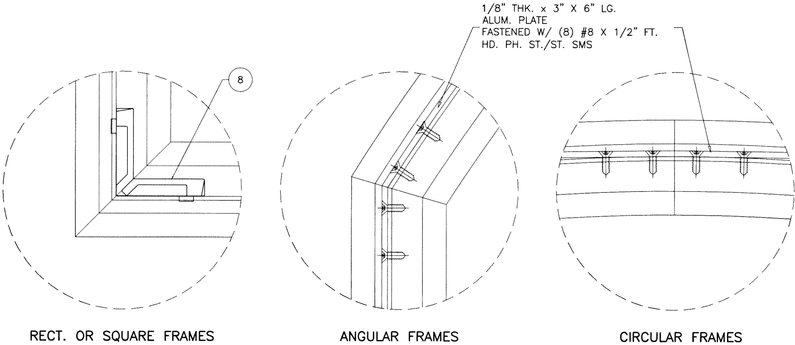
WINDOW CORNER DETAILS
