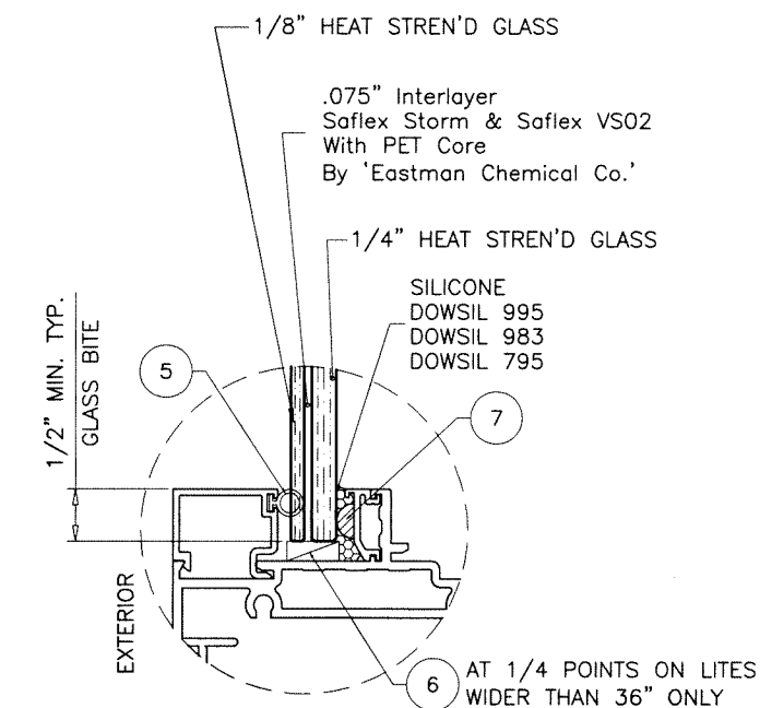
GLASS TYPE 'C' 7/16" OVERALL LAM. GLASS
